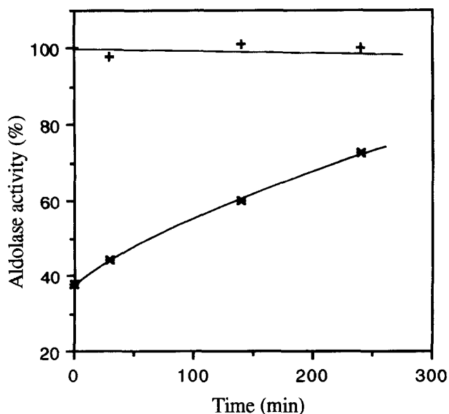
Figure 4. Partial reversion of aldolase inhibition by compound 3 in the presence of p -phenyldiphosphate. (*) aldolase inhibited by compound 3; (+) control. Aldolase (10 mg mL -1 , TEA buffer pH 7.60, rt) was incubated with 3 mM compound 3 until 62% loss activity, then diluted 100-fold in TEA buffer containing p -phenyldiphosphate (5 mM) at 25 °C. At various times, residual activity was determined on 20 \mu L aliquots (see Experimental). The control was run without compound 3. After a 24 h incubation with a competitive inhibitor, 80% of the initial activity was recovered.
