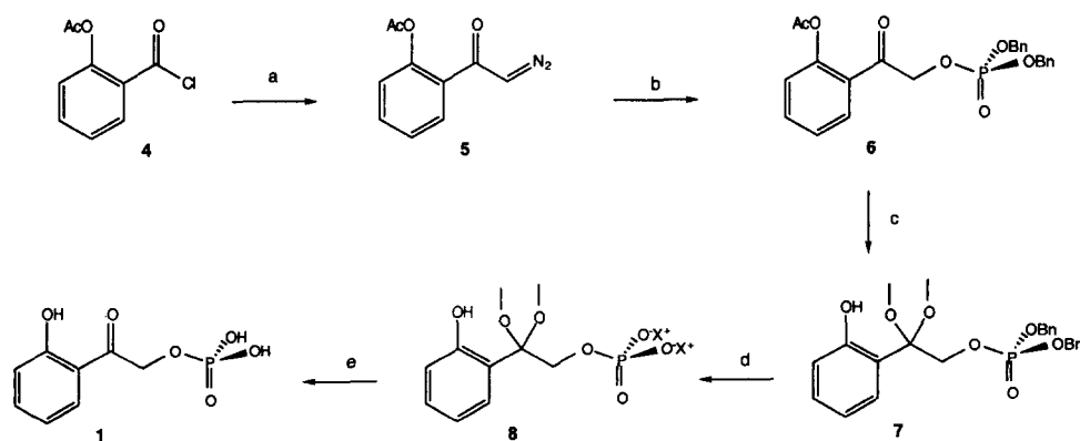
Scheme 3. Synthetic scheme for the synthesis of compound 1 . (a) \text{CH}_3\text{N}_2 ; (b) (\text{BnO})_2\text{P}(\text{O})\text{OH} ; (c) \text{HC}(\text{OMe})_2 , \text{MeOH} , \text{H}^+ ; (d) (1) \text{H}_2 , \text{Pd/C} (2) \text{C}_6\text{H}_{11}\text{NH}_2 ; (e) \text{H}_2\text{O} , Dowex \text{H}^+ .
